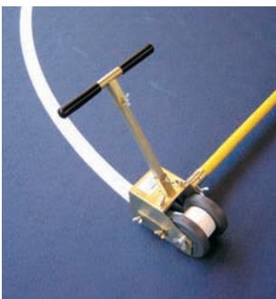
Marking Head with 50 mm marking tape
