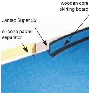
Fitting of wooden core skirting boards with Jantac Super 35.
