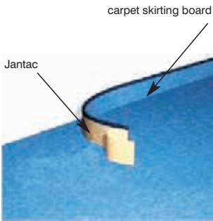
Fitting of carpet skirting boards with Jantac.
