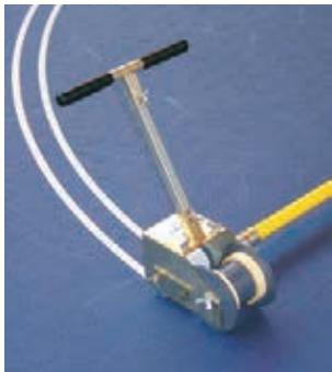
Marking Head with 19 mm masking tape
